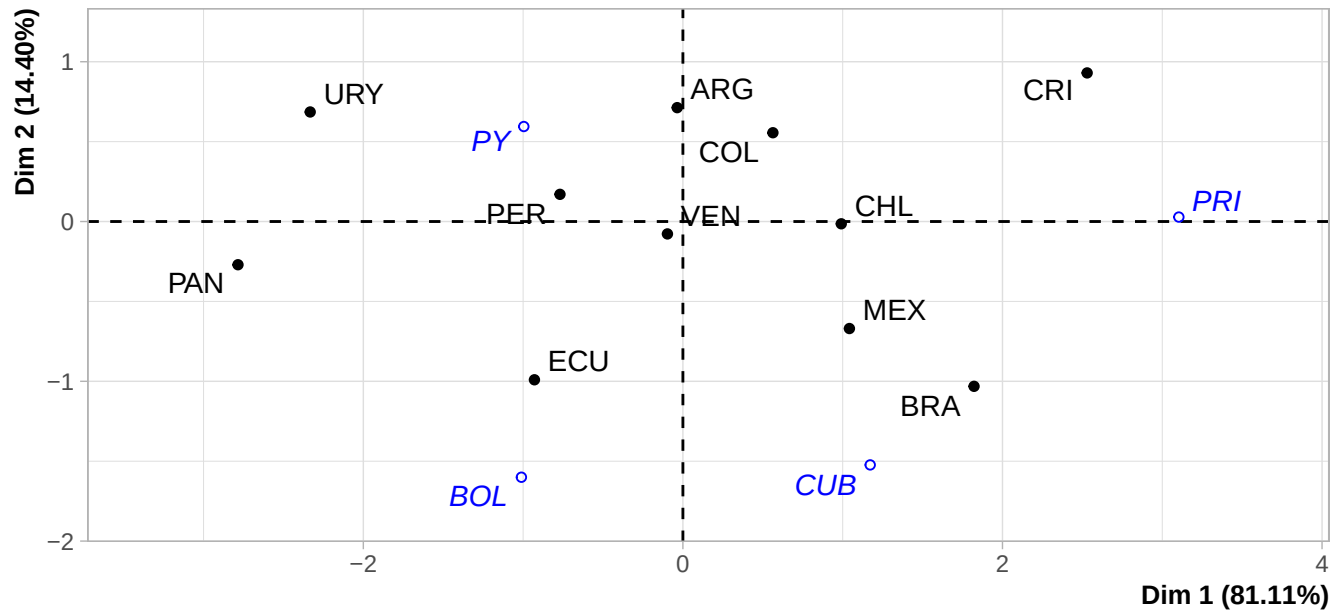
PCA graph of individuals
