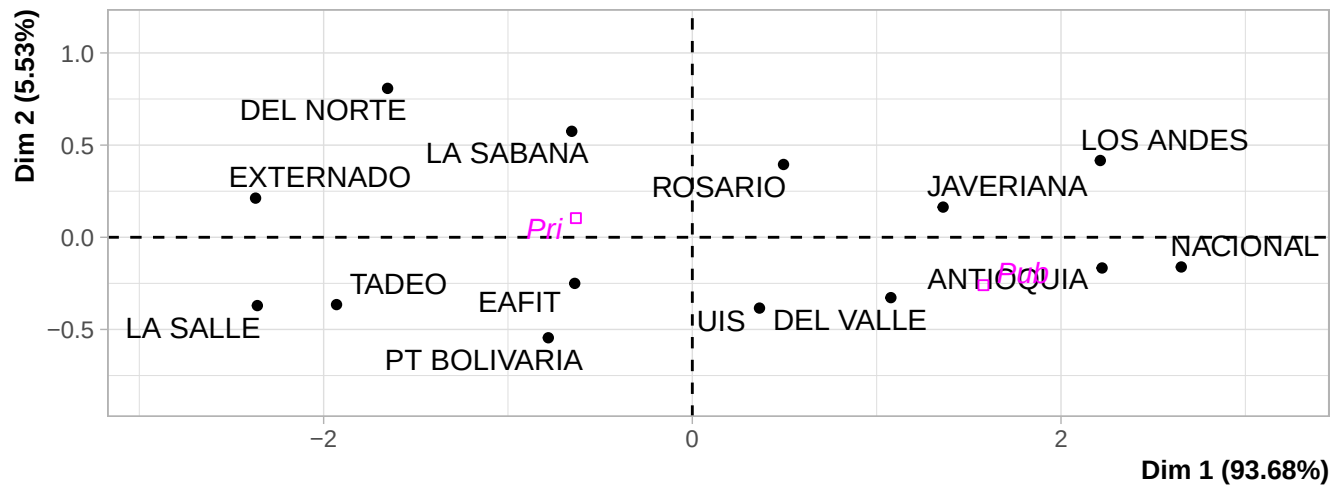
PCA graph of individuals
