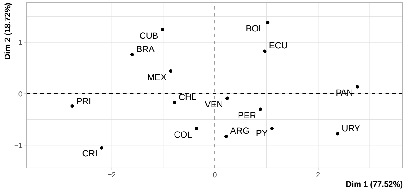
PCA graph of individuals
